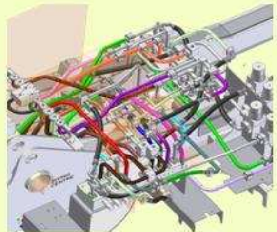
HYDRAULIC PIPING LAYOUT
